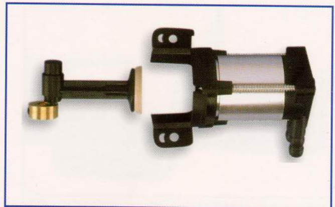
DETAIL OF THE ALUMINIUM CYLINDER AND THE ECCENTRIC/ROD PATENT LUBRICATION SYSTEM
